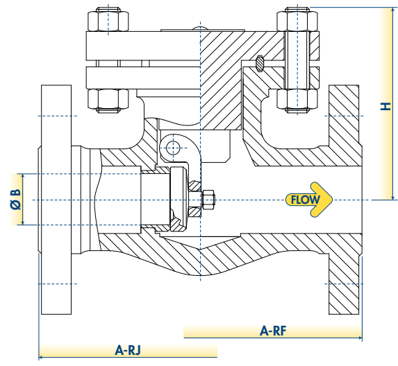
DESIGN TYPE S2 RING JOINT BODY-BONNET CONNECTION
